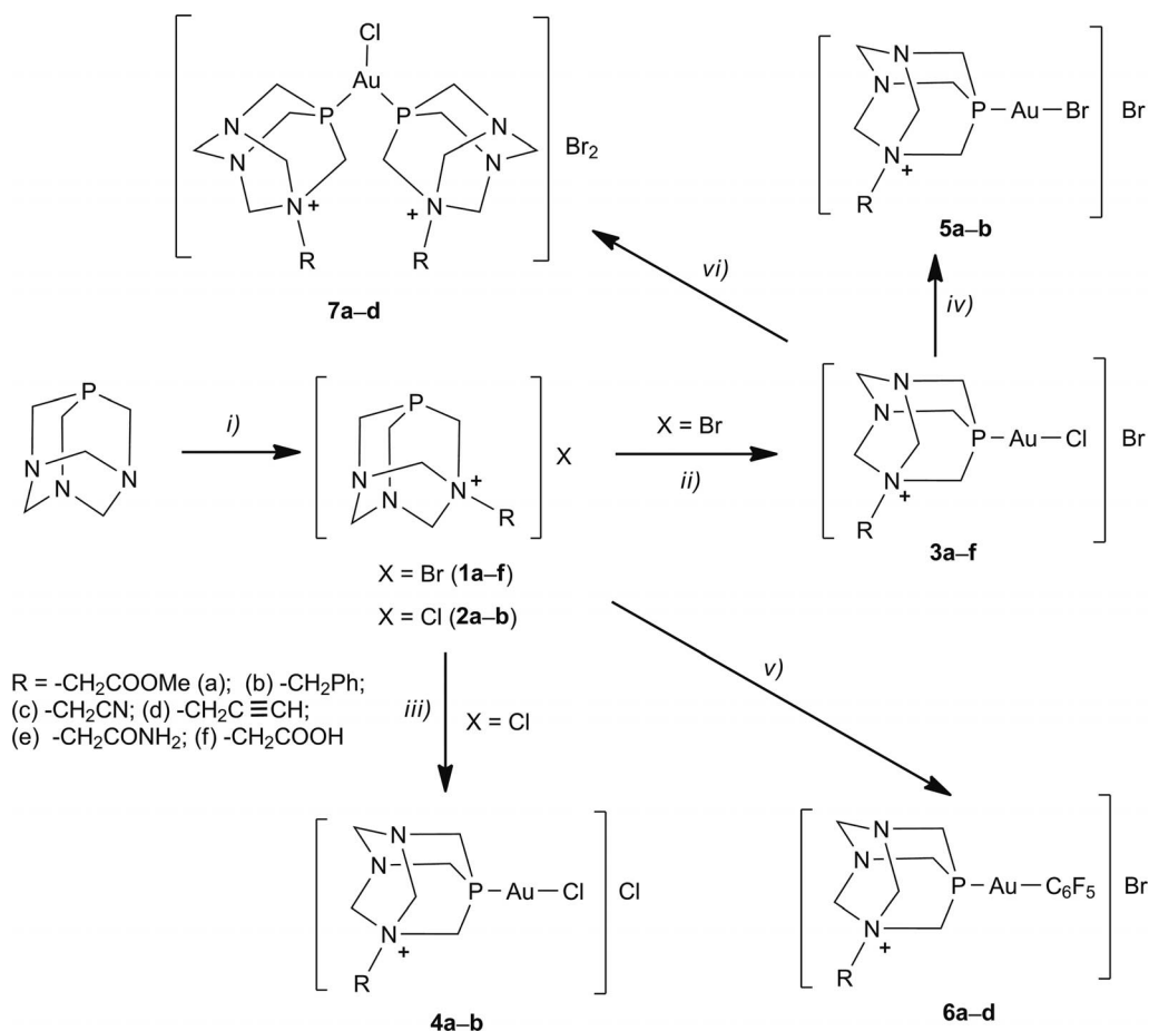
Scheme 1. (i) RX, (ii, iii) [AuCl(tht)], (iv) NaBr, (v) [Au(C 6 F 5 ) 3 (tht)] and (vi) [PTA–R]X.
