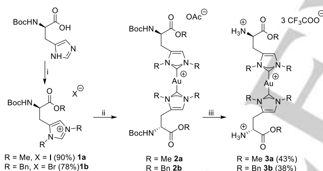
Scheme 1: Synthesis of imidazolium salts 1a and 1b ; and of Au(I) bis-NHC complexes 2a , 2b (not isolated), 3a and 3b . i: NaHCO 3 , RX, 110 °C, 16 h (MeCN); ii: 1. Ag 2 O, Au(THT)Cl (THT = tetrahydrothiophene), r.t. 16 h (DCM); 2. AgOAc, 15 min, r.t., 3. TFA/DCM (5/1), r.t. 2 h.
