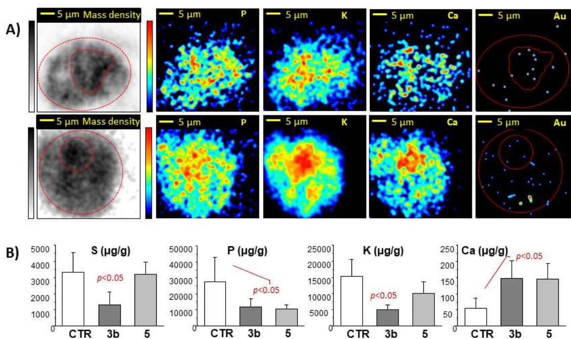
Figure 3: A) Mass density and elemental maps of spatial distribution of P, K, Ca and Au in individualized PC3 treated cells by nuclear microscopy: complexes 3b (upper panel) and 5 (lower panel) complexes. The dotted lines in mass and Au maps indicate the cell contour and the nuclear region. The mass density and elemental distribution are represented by a colour gradient with a dynamic scale: high level- black/red; low level- white/deep blue. B) Concentrations of S, P, K and Ca (µg/g dry weight) in cells. Significant differences indicated ( p < 0.5 ) relative to controls (non-treated cells).
