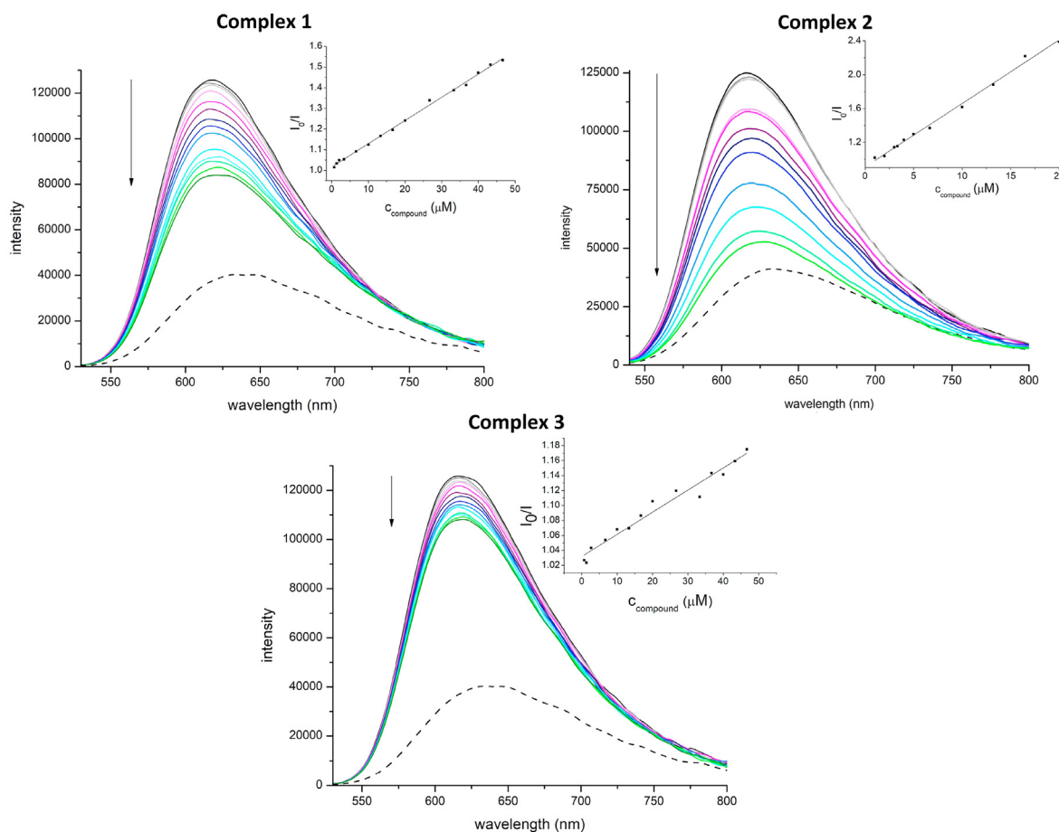
Fig. 5. Emission spectra ( \lambda_{\text{ex}} = 510 \text{ nm} ) of EB–CT–DNA in PBS buffer with the increasing concentration of 1–3 (0–50 \mu\text{M} for 1, 3 and 0–20 \mu\text{M} for 2 ). The inset shows the Stern–Volmer plots for corresponding complexes.
