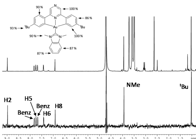
Figure 6. Interaction of 2 with MDM2 in solution studied by STD NMR ( 13.5 \mu\text{M} MDM2, 500 \mu\text{M} 2 , 1% DMSO- d_6 , 800 MHz, 25^\circ\text{C} ). (top) ^1\text{H} NMR reference spectrum. The inset shows the group epitope mapping of 2 from STD NMR experiments derived from STD NMR intensities at very low saturation time (0.5 s). Ligand hydrogens showing high % values have close contacts with the surface of the binding pocket of MDM2. (bottom) STD NMR spectrum (4 s saturation time) showing signals of 2 resulting from the binding in solution (intense signals around 3.5–3.7 ppm in the reference spectrum belong to glycerol, which does not bind to MDM2).
