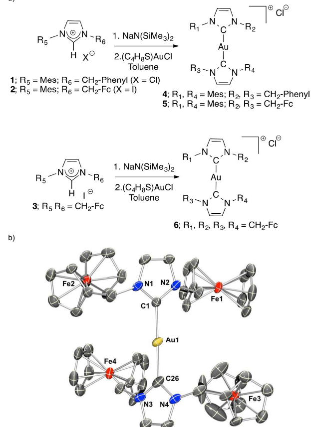
Figure 2. a) Synthesis of ferrocene containing Au(I) carbene complexes. b) ORTEP diagram of 6 rendered using POV-Ray. Thermal ellipsoid plots are drawn at the 50% probability level. Hydrogen atoms and counter anion are omitted for clarity. Selected bond lengths (Å) and angles (deg): C1–N1, 1.37(1); C1–N2, 1.35(2); C1–Au1, 2.021(9); C26–Au1, 2.028(8); C26–N3, 1.33(1); C26–N4, 1.35(1); N1–C1–N2, 105.2(8); N3–C26–N4, 105.1(7); C1–Au1–C26, 176.5(3).
