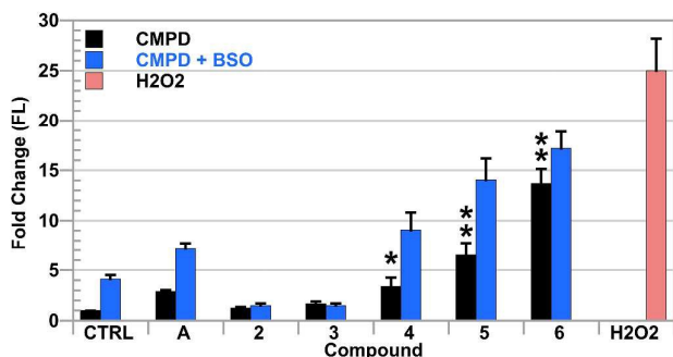
Figure 5. Reactive oxygen species detected by fluorescent signal increases of DCF via flow cytometric analysis in live A549 cells treated with various complexes. H 2 O 2 was used as a positive control. Error bars represent one standard deviation. A one-way ANOVA with Dunnett's post-hoc test was used to compare each compound with the vehicle control (* P <0.05; ** P <0.01).
