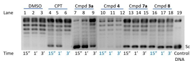
Figure 4. Inhibition of TopI activity along the time (15", 1' and 3') by compounds 3a , 4 , 7a and 8 and camptothecin at 100 \mu M: lanes 1-3, DNA+TopI+DMSO; lanes 4-6, DNA+TopI+camptothecin 100 \mu M; lanes 7-9, DNA+TopI+ 3a 100 \mu M; lanes 10-12, DNA+TopI+ 4 100 \mu M; lanes 13-15, DNA+TopI+ 7a 100 \mu M; lanes 16-18, DNA+TopI+ 8 100 \mu M; lane 19, control DNA. Reaction samples were mixed with enzyme at 37°C before adding the supercoiled DNA substrate and separated by electrophoresis on a 1% agarose gel, and then stained with gel red, and photographed under UV light as described in the TopI mediated DNA relaxation assay.
