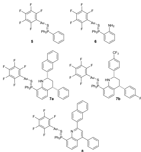
Chart 1. Gold(I) complexes 5-8 .
