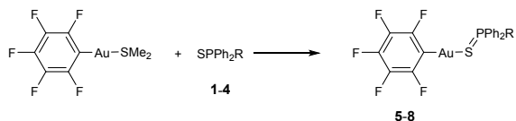
Scheme 2. Syntheses of gold(I) complexes 5-8 .
