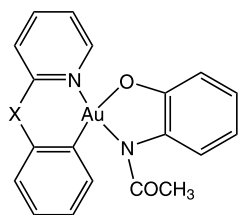
7a , X = NH 7b , X = CH 2
