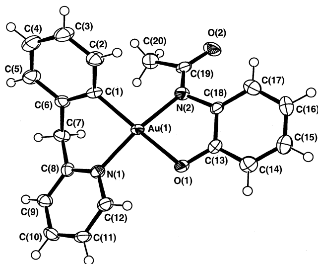
Fig. 1. Molecular structure of molecule 1 of [(2-benzylpyridyl)-Au{N(COCH 3 )C 6 H 4 O}] ( 7b ) showing the atom numbering scheme. Thermal displacement ellipsoids are depicted at the 50% probability level.
