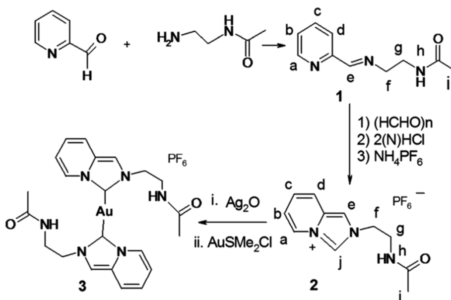
Figure 1 Synthesis of the gold(I) N-heterocyclic carbene complex 3 .
