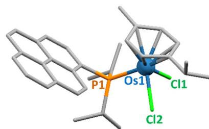
Fig. 3 Representation of the crystal structure of \text{Os}_{\text{Cl}_2}^{\text{iPr}} . The atoms bonded to the metal centre are labelled. Hydrogen atoms are omitted for clarity.
