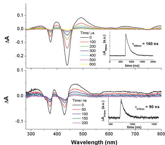
Fig. 12 Nanosecond time-resolved absorption difference spectra of 2a in O_2 -saturated MeCN (top) and 2c in O_2 -saturated DMF (bottom). Inset: decay kinetic of absorption difference at 490 nm (top) and 470 nm (bottom).
