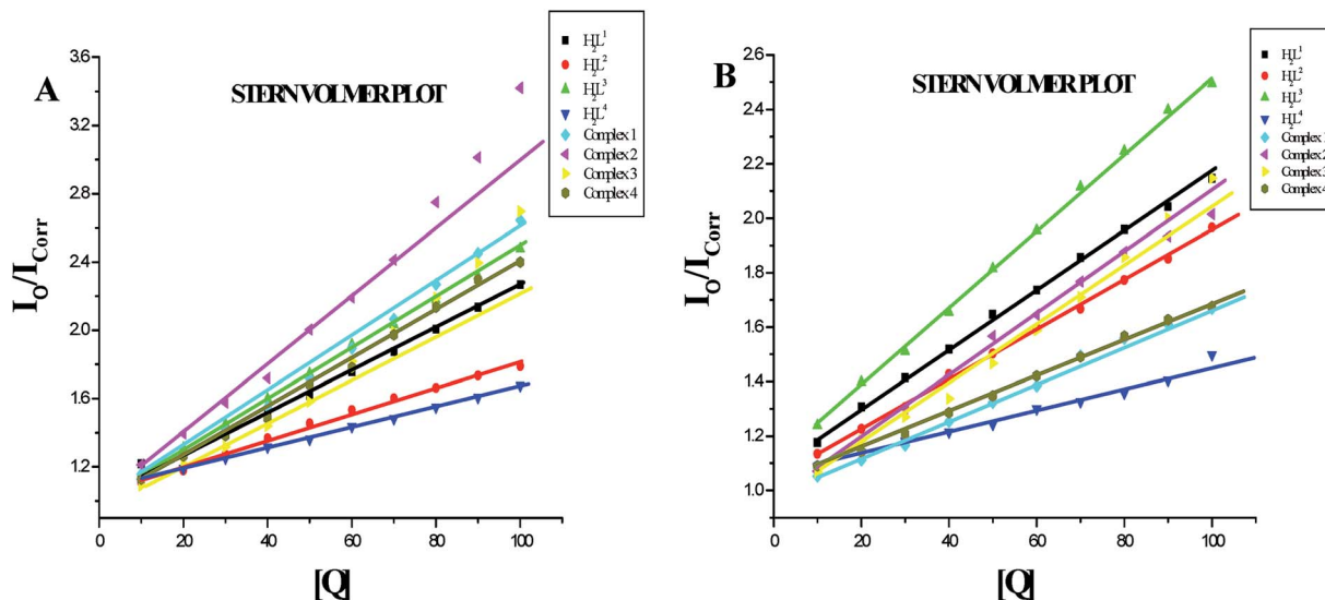
Fig. 13 (A) Stern–Volmer plot of the fluorescence titration of the ligands H_2L^{1-4} and complexes (1–4) (10–100 μM) with BSA (10 μM). (B) Stern–Volmer plot of the fluorescence titration of the ligands H_2L^{1-4} and complexes (1–4) (10–100 μM) with HSA (10 μM).
