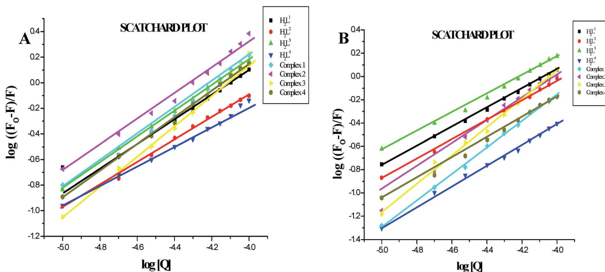
Fig. 14 (A) Scatchard plot of the fluorescence titration of the ligands H_2L^{1-4} and complexes (1–4) (10–100 μM) with BSA (10 μM). (B) Scatchard plot of the fluorescence titration of the ligands H_2L^{1-4} and complexes (1–4) (10–100 μM) with HSA (10 μM).
