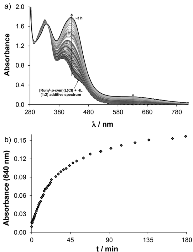
Fig. 7 Time-dependent UV-Vis absorption spectra of the [Ru( \eta^6 - p -cym)(L)(H 2 O)] + -HQCl-Pro (1:2) system at pH = 7.40 in the presence of O 2 (L: the coordinated form of HQCl-Pro). The dashed curve shows the additive spectrum of the metal complex and 2 equivalents of the HQCl-Pro ligand. The inserted figure shows absorbance values at 640 nm as a function of time. {c([Ru( \eta^6 - p -cym)(L)(H 2 O)] + ) = 200 \mu M; c(HQCl-Pro) = 400 \mu M; pH = 7.40 (20 mM phosphate); c(KCl) = 0.10 M; T = 25.0 ^{\circ} C; l = 1 cm}.
