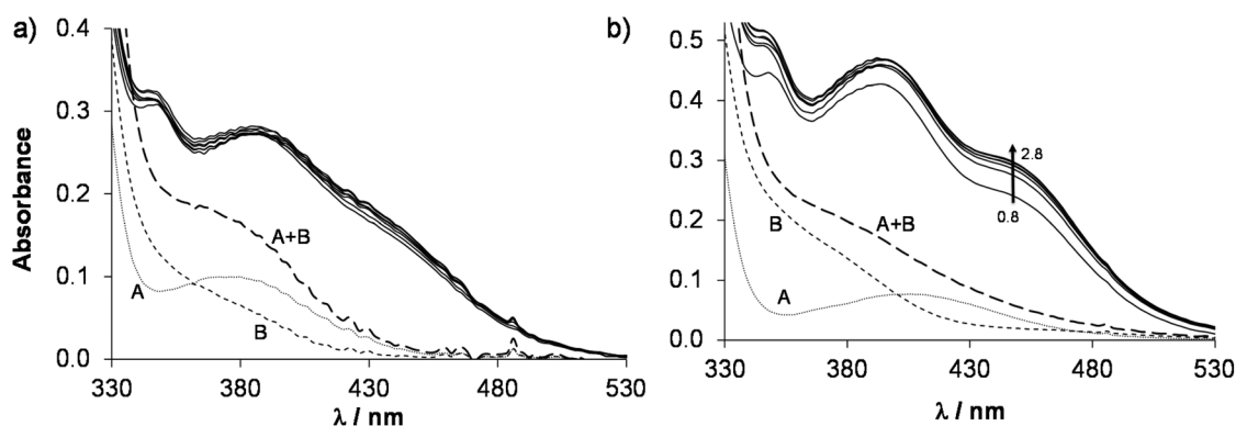
Fig. 5 UV-Vis absorption spectra (solid lines) of the (a) \text{Rh}(\eta^5\text{-C}_5\text{Me}_5) -HQCl-Pro system at \text{pH} = 0.8\text{--}2.0 and of the (b) \text{Ru}(\eta^6\text{-p-cym}) -HQCl-Pro system at \text{pH} = 0.8\text{--}2.8 . The dotted curve shows the absorption spectrum of the free organometallic cation (A), the dashed curve (B) shows the spectrum of the free HQCl-Pro ligand and the long dashed curve (A + B) shows their additive spectrum. \{c([\text{Rh}(\eta^5\text{-C}_5\text{Me}_5)(\text{H}_2\text{O})_3]^{2+}) = c(\text{HQCl-Pro}) , in Fig. 4a) = 60 \mu\text{M} ; c([\text{Ru}(\eta^6\text{-p-cym})(\text{H}_2\text{O})_3]^{2+}) = c(\text{HQCl-Pro}) , in Fig. 4b) = 115 \mu\text{M} ; I = 0.20 \text{ M (KNO}_3) ; T = 25.0 \text{ }^\circ\text{C} ; l = 1 \text{ cm} .
