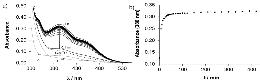
Fig. 3 (a) Time-dependent UV-Vis absorption spectra of the Ru(η 6 -tol)-HQCl-Pro (1 : 1) system at pH = 3.64 (solid lines). Dotted curves show the absorption spectra of the triaqua organometallic metal ion (A) and HQCl-Pro ligand (B); the dashed curve shows their additive spectrum (A + B). (b) Absorbance values at 388 nm as a function of time. {c([Ru(η 6 -tol)(H 2 O) 3 ] 2+ ) = c(HQCl-Pro) = 101 μM; pH = 3.65; I = 0.20 M (KNO 3 ); T = 25.0 °C; ℓ = 1 cm}.
