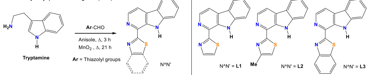
Chart of Thiazolyl- \beta -carboline Ligands ( N^*N' )
