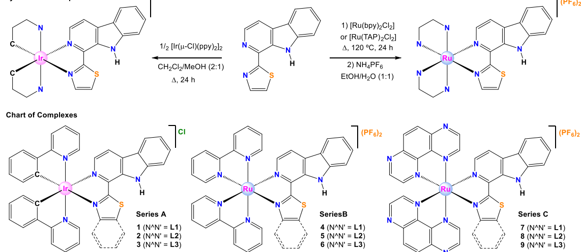
Scheme 2. Synthesis of complexes with L1 as illustrative examples and molecular structure of complexes 1–9.
