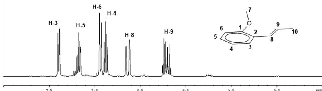
Fig. 3. ^1\text{H} NMR spectra of compound 3 (a) and free 2-(1-propenyl)anisole (b).
