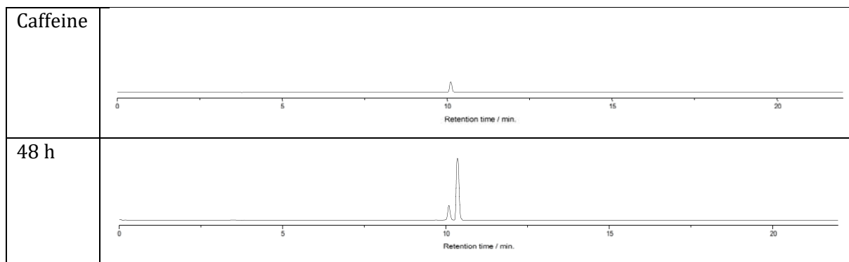
Figure S38. HPLC chromatogram (Method M1) of Caffeine (internal standard) and 4 after 48 h incubation in human pooled plasma.
