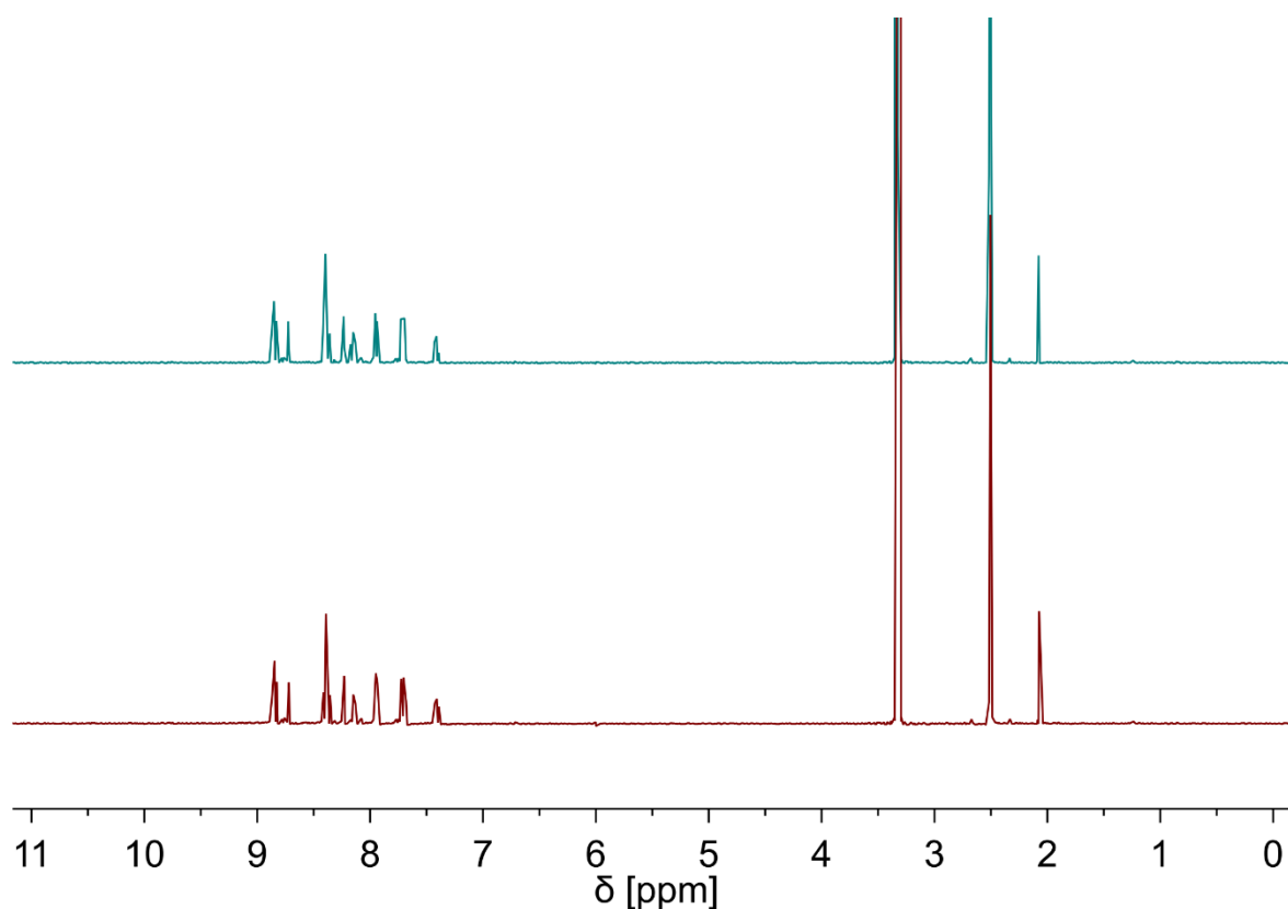
Figure S28. 1 H NMR spectrum of 1 in DMSO-d 6 after preparation (green) and 7 days (red).
