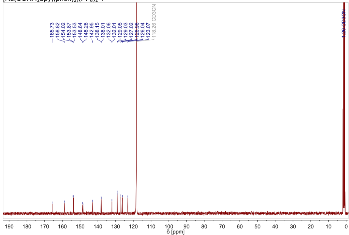
Figure S8. 13 C NMR spectrum of 4 in CD 3 CN, 100 MHz.
