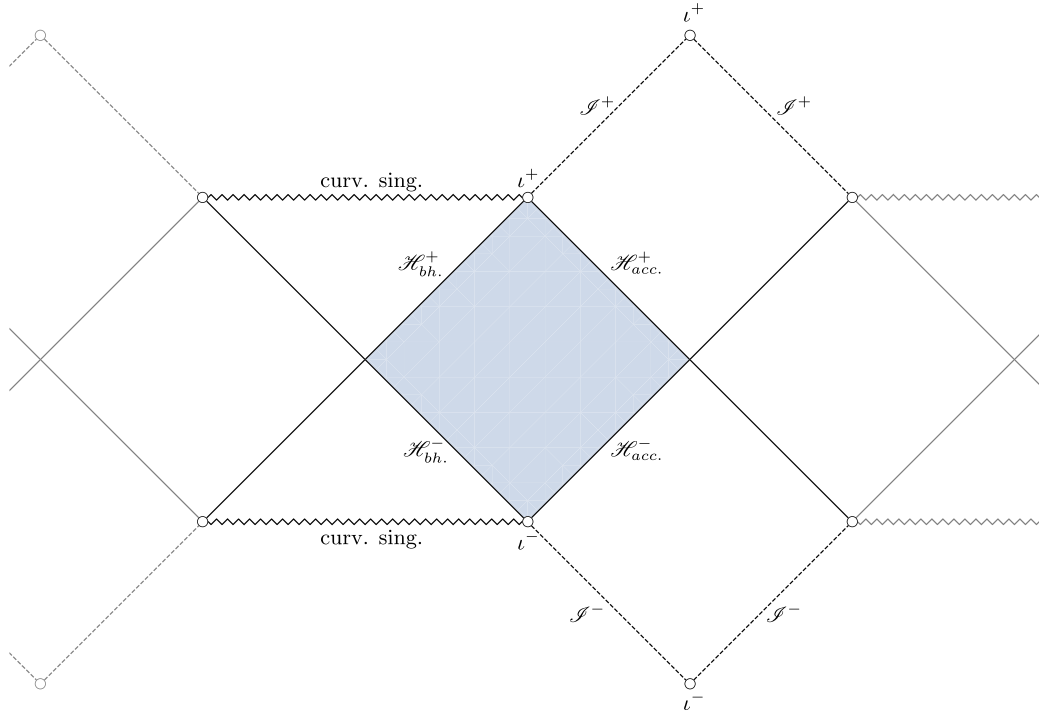
Fig. 1. A section of the Penrose diagram of the maximally analytically extended uncharged C-metric without cosmological constant. The shaded region corresponds to a static patch.
