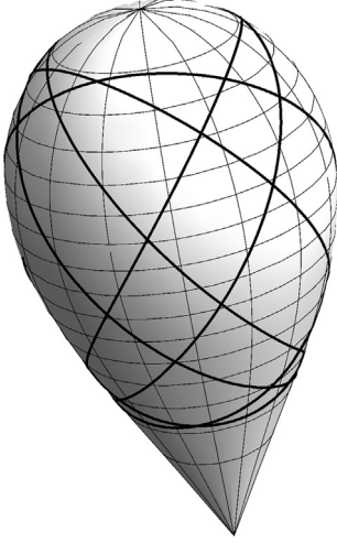
Fig. 2. The photon surface for the C-metric with ma = 0.2 , showing a portion of a geodesic.
