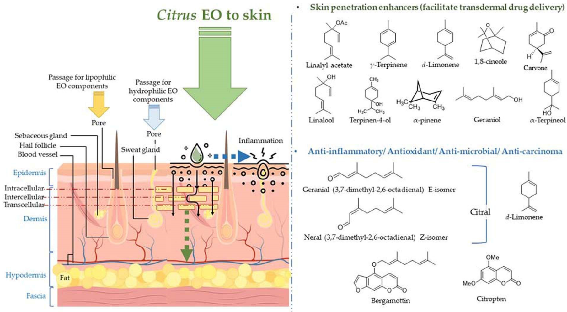
Figure 6. Absorption of citrus EOs to the deeper layers of the skin, molecular structures of the skin penetration enhancers (frequently employed in topical lotions/ointments for facilitating transdermal drug delivery), and molecules participating in anti-inflammatory, anti-microbial, and anti-carcinoma activities.
