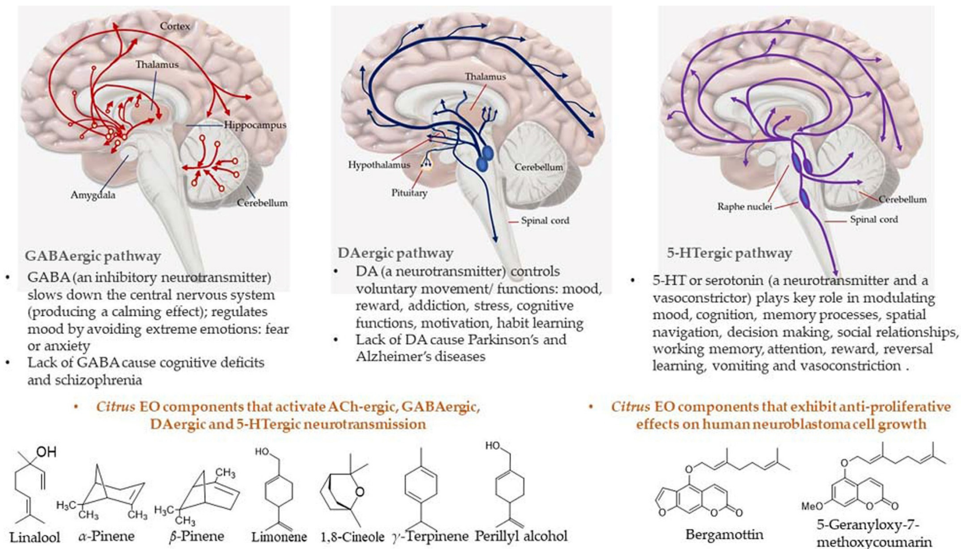
Figure 15. Neurotransmission pathways in GABAergic, DAergic, and 5-HTergic neurons and Citrus EO components that activate neurotransmission and exhibit anti-proliferative effects on human neuroblastoma cell growth.
