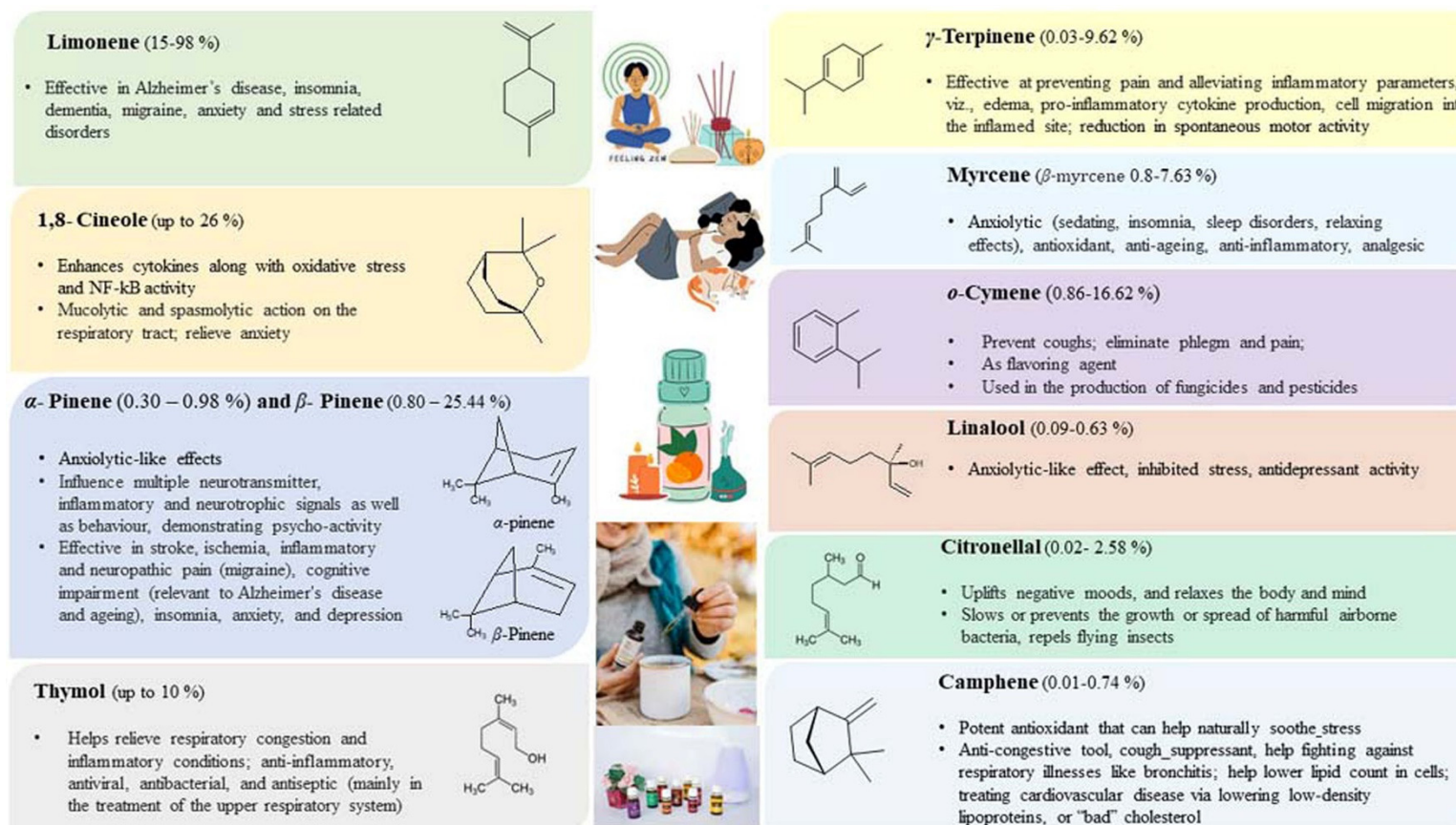
Figure 16. Therapeutic effects of majorly occurring component in citrus essential oil [202,208–211].
