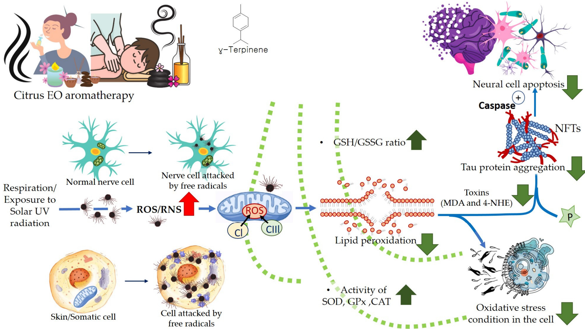
Figure 9. Therapeutic effect of citrus EOs aromatherapy.
