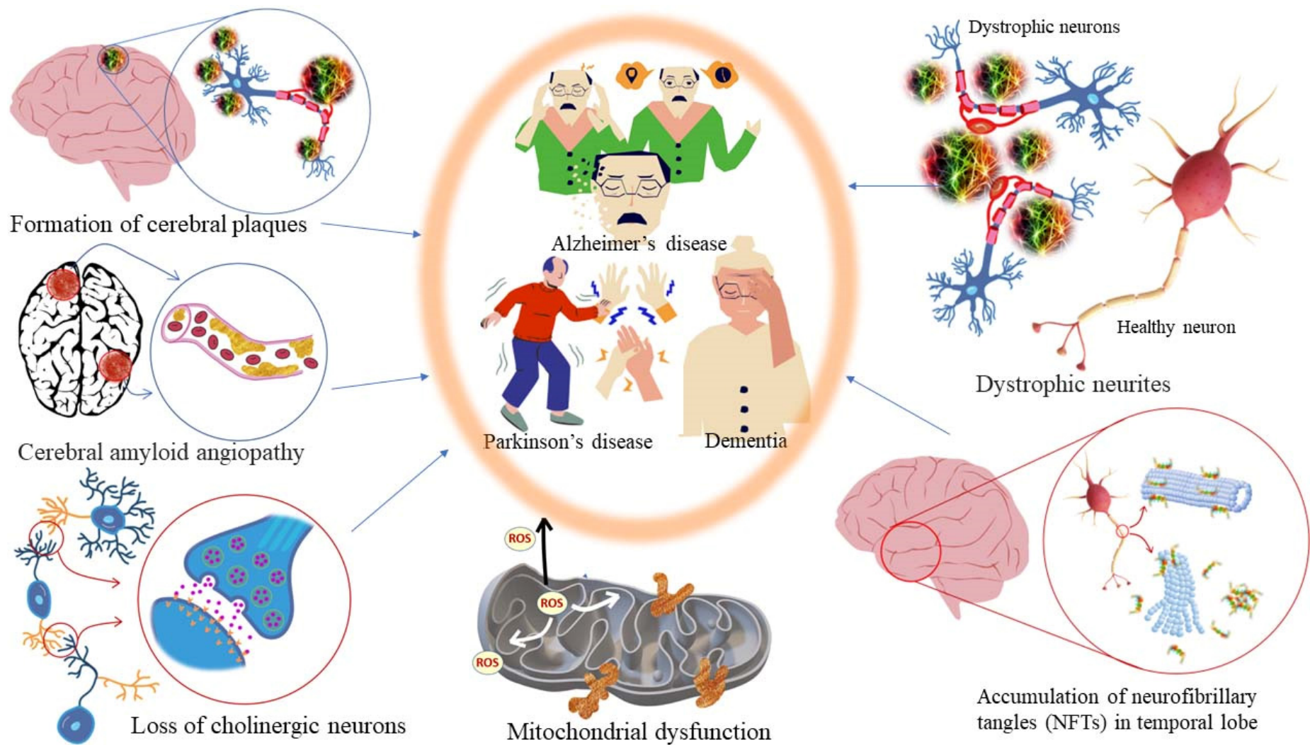
Figure 12. Pathological targets in diseased conditions of dementia, Alzheimer's, and Parkinson's.
