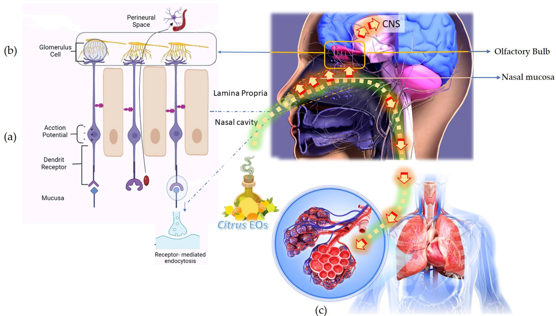
Figure 3. Inhalation of the citrus EOs and response delivery to the central nervous system through the olfactory lobe and respiratory and circulatory system. (a) Activation of nasal olfactory chemoreceptors (b) Direct absorption of the EO active molecules into the neuronal pathway (c) Absorption of EO active molecules in the alveolar blood circulation.
