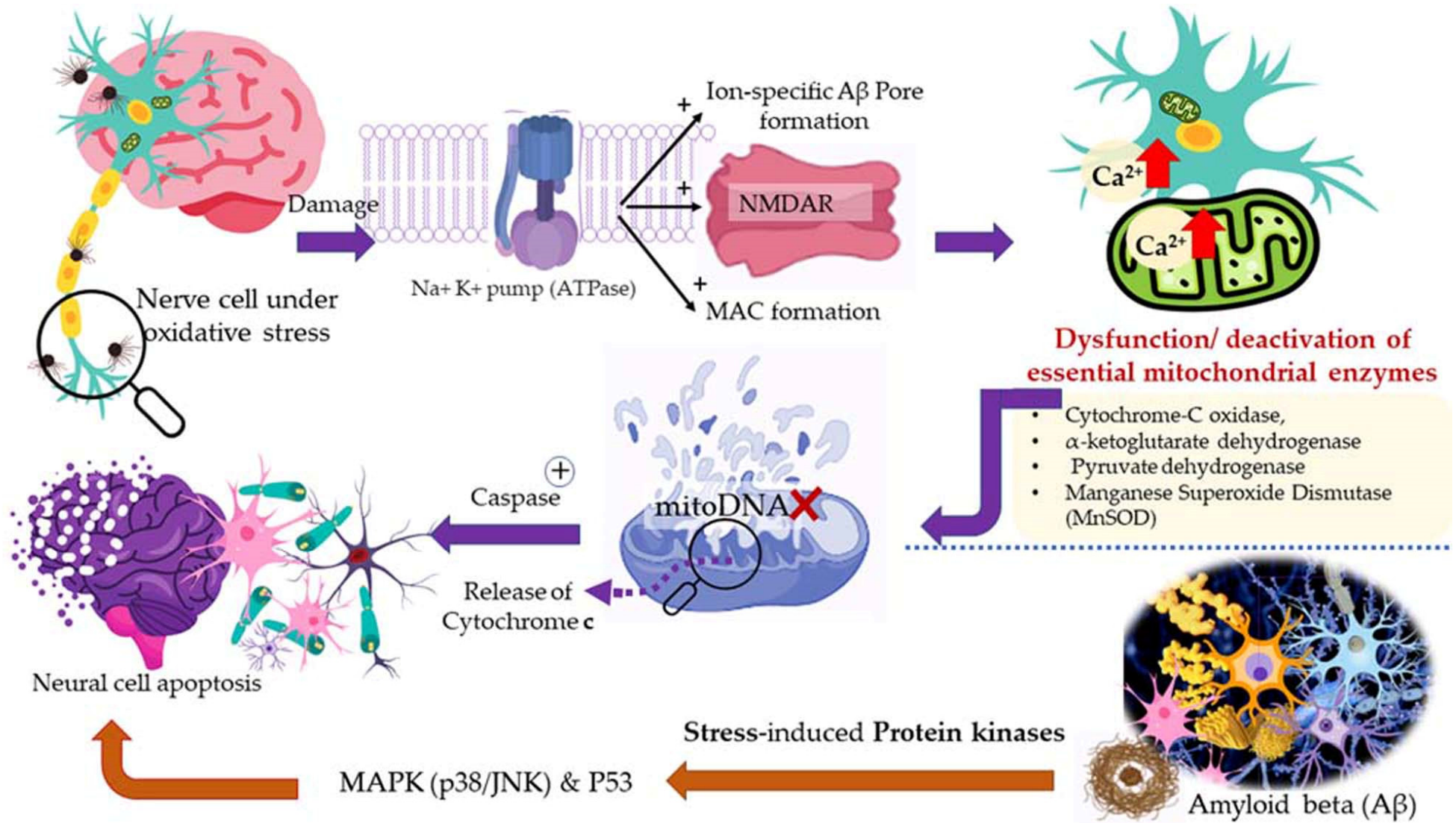
Figure 8. Oxidative stress in the cell: Events and consequences-II: Nerve cell.
