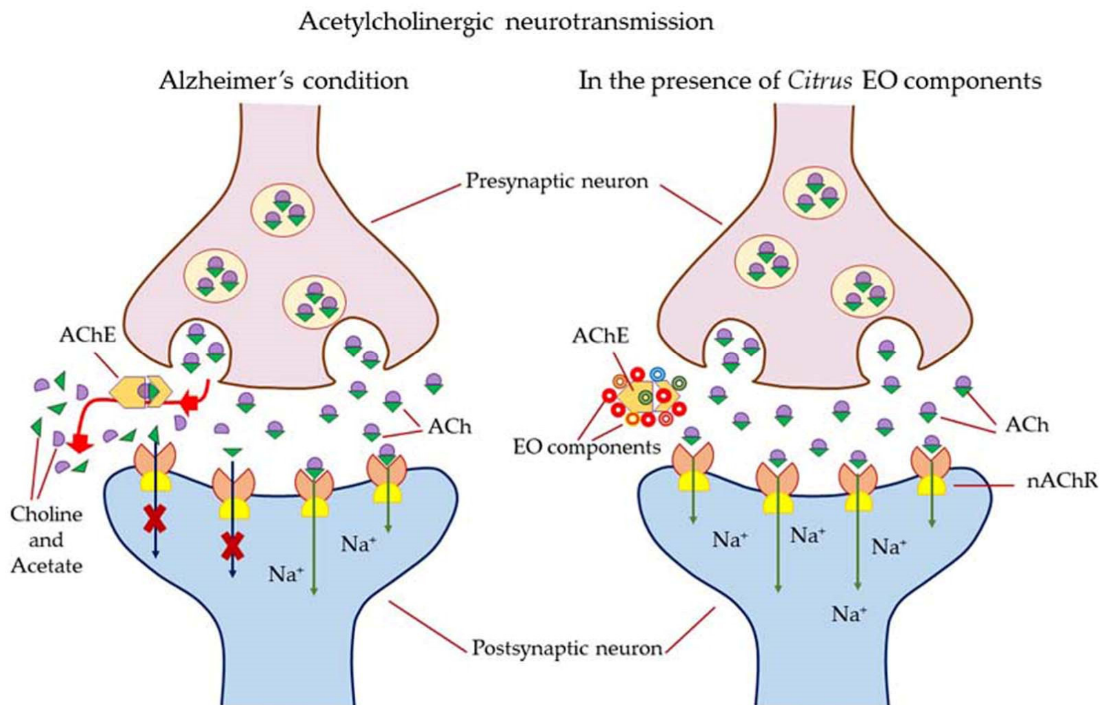
Figure 13. Mechanism of action of citrus EOs to inhibit acetylcholinesterase (AChE), thereby increasing levels and duration of acetylcholine in the brain and assisting with cognition (learning and memory retention). Abbreviation; ACh—acetylcholine; AChE—acetylcholinesterase; nAChR—nicotinic acetylcholine receptors; EOs—Citrus essential oil components.
