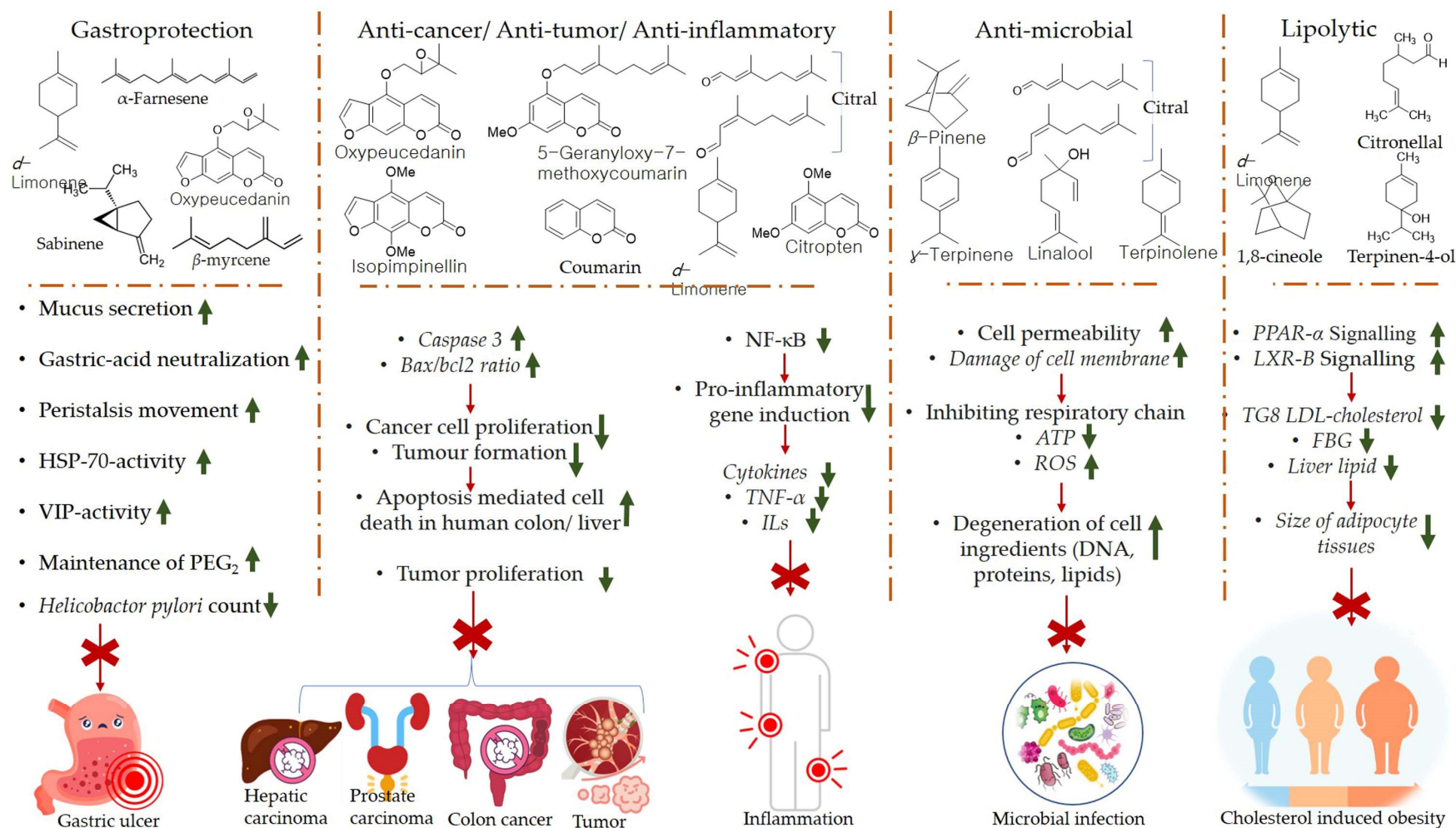
Figure 5. Mechanisms of gastroprotection, anti-cancer, anti-tumor, anti-inflammation, anti-microbial, and lipolytic actions of citrus EO components. Caspase (key apoptosis-inducing protein) [85–92]. Abbreviations; PPAR- \alpha (Peroxisome proliferator-activated receptor alpha), bcl 2 (B-cell lymphoma protein 2), Bax (bcl 2-associated X), NF- \kappa B (Nuclear factor- \kappa B), LXR- \beta (Liver X receptor beta), TG8 LDL (Triglycerides 8 Low-density lipoprotein), FBG (fasting blood glucose), ROS (Reactive Oxygen Species), TNF- \alpha (tumor necrosis factor alpha), ILs (Interleukins), ATP (Adenosine triphosphate).
