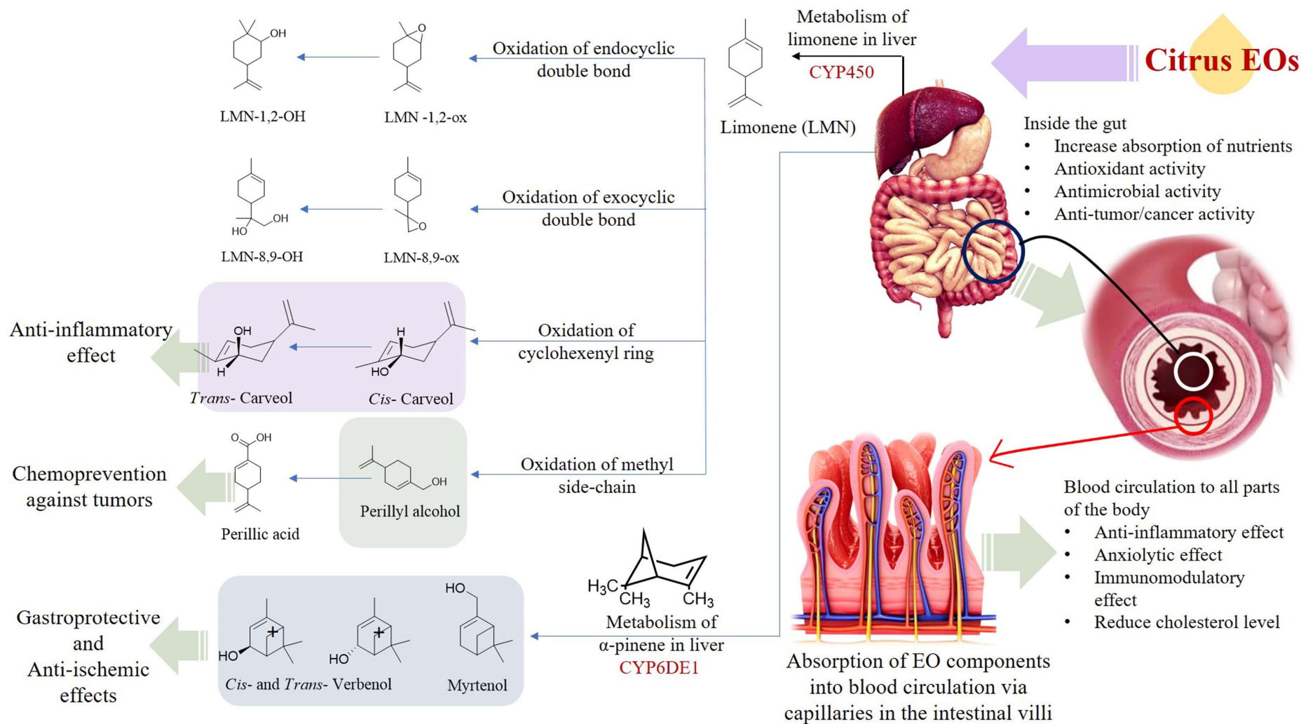
Figure 4. Metabolism of d -limonene and \alpha -pinene in the liver, absorption of citrus EO components into the circulatory system through the intestinal villi.
