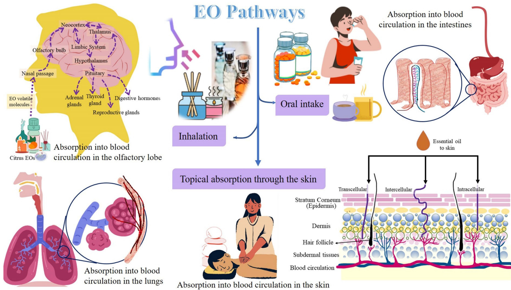
Figure 2. Pathways followed by citrus EOs for aromatherapy.
