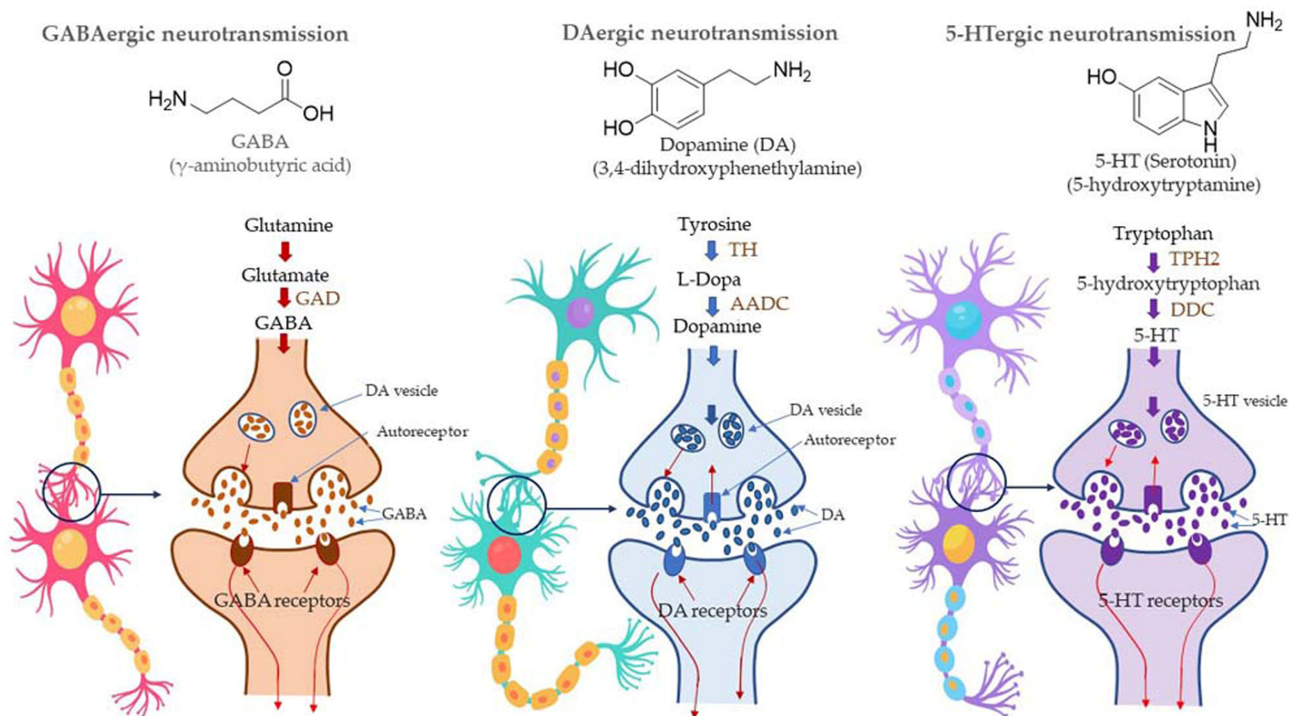
Figure 14. Syntheses of neurotransmitter molecules, viz., GABA ( \gamma -Aminobutyric acid), dopamine, and serotonin (also called as 5-HT) and the mechanism of neurotransmission. AADC also known as DDC. Abbreviations; GAD (glutamate decarboxylase), TH (Tyrosine hydroxylase), AADC (aromatic amino acid decarboxylase), DDC (DOPA decarboxylase), TPH2 (tryptophan hydroxylase 2).
