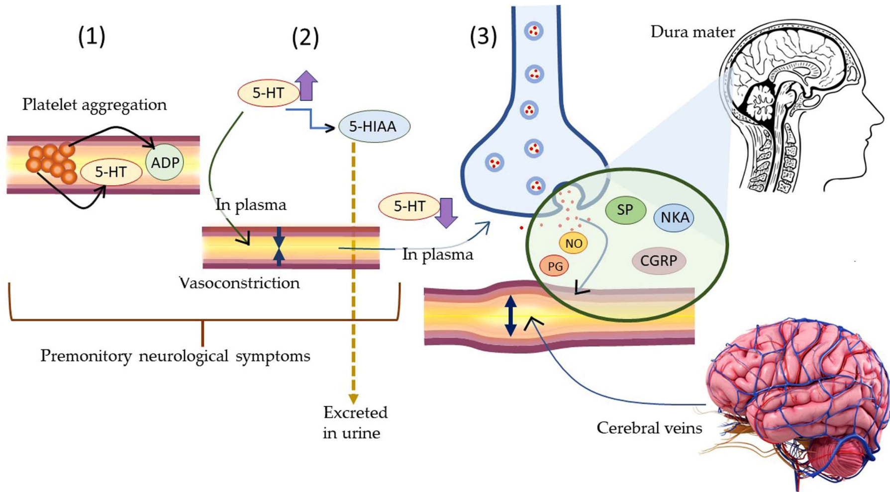
Figure 10. The pathophysiological mechanism of migraine induced by 5-HT. (1) Platelet aggregation trigger release of 5-HT and ADP in blood plasma. (2) High level of plasma 5-HT causes reversible vasoconstriction followed by conversion of 5-HT to its metabolite 5-HIAA. The latter is excreted in urine. (3) Low level of plasma 5-HT stimulates perivascular neurons to release neuropeptides (NO, PG, SP, NKA, CGRP) causing vasodilation of cerebral veins. The latter leads to migraine symptoms.
