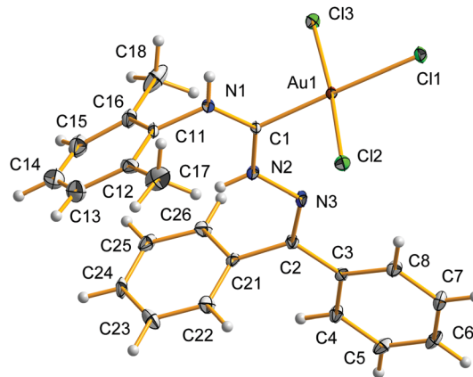
Fig. 1 Crystal structure of 14 with the atomic numbering scheme (hydrogen labels and chloroform molecules were omitted for simplicity). Thermal ellipsoids are drawn at the 25% probability level. Selected bond lengths (Å) and angles (°): Au1–Cl1 2.3255(12), Au1–Cl2 2.2687(14), Au1–Cl3 2.3001(14), Au1–C1 2.005(5), C1–N1 1.312(6), C1–N2 1.318(5), C2–N3 1.293(6), N2–N3 1.387(5), C1–Au1–Cl1 178.55(12), C1–Au1–Cl2 87.21(16), C1–Au1–Cl3 89.29(16), Cl1–Au1–Cl2 92.63(5), Cl2–Au1–Cl3 175.16(5), N1–C1–Au1 121.9(3), N1–C1–N2 118.4(4), N2–C1–Au1 119.7(3).
